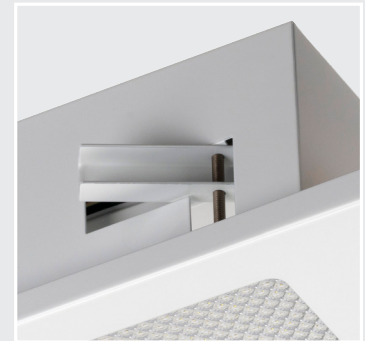
ADJUSTABLE CEILING BRACKETS
