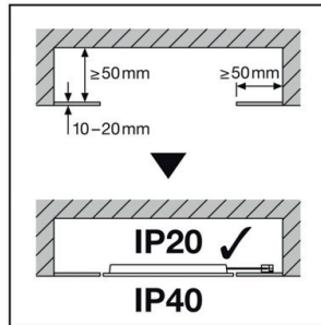
Minimum Insulation Spacing
